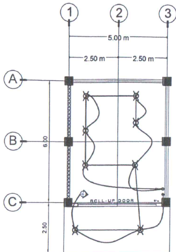
LIGHTING LAYOUT PLAN SCALE 1:80
