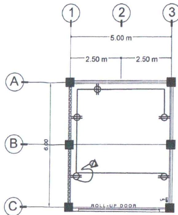
POWER LAYOUT PLAN SCALE 1:80
