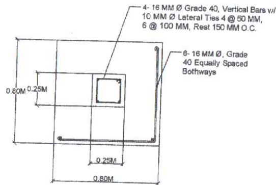
C1F1 DETAIL
