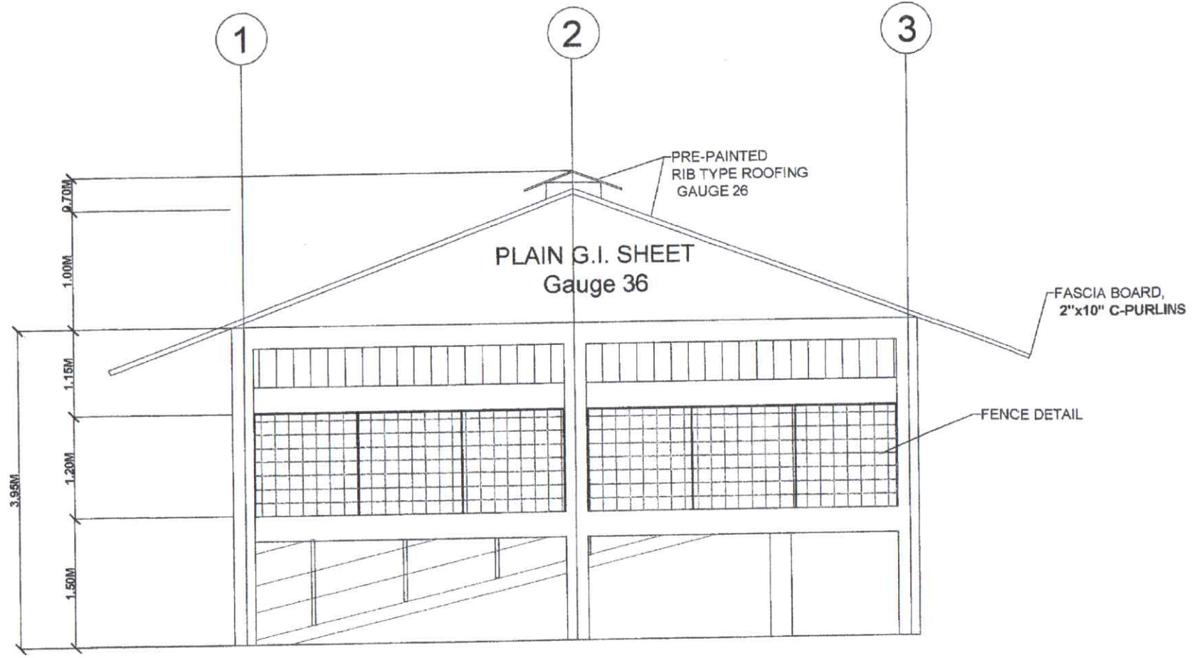
REAR VIEW ELEVATION Scale NTS
