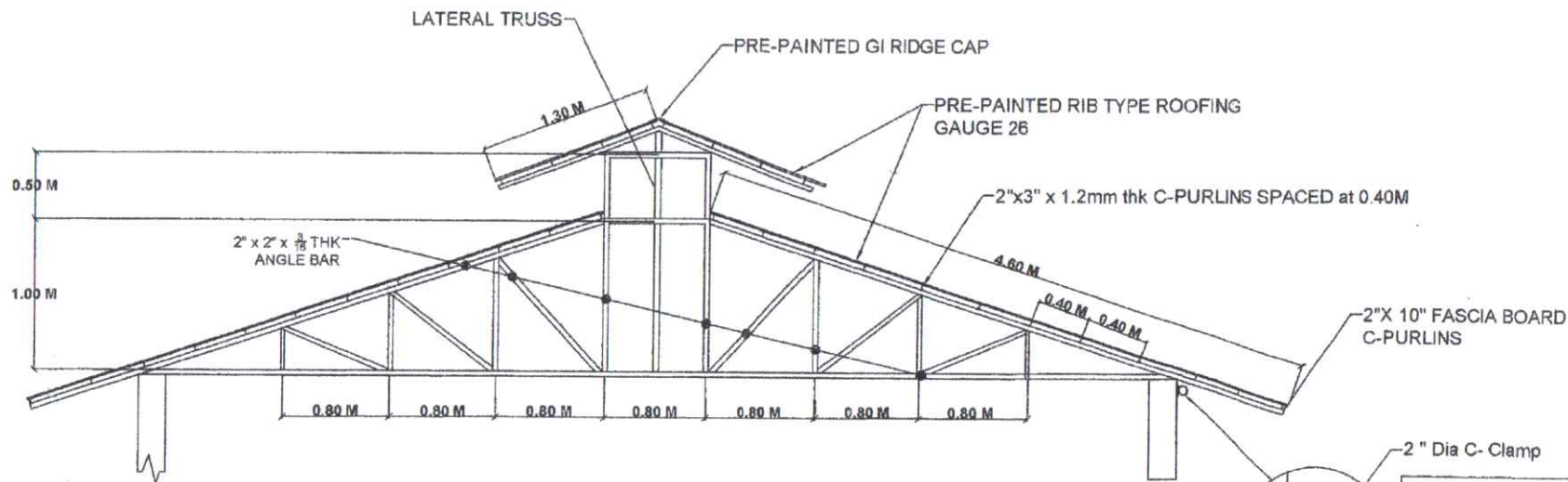
TRUSS DETAIL Scale NTS
