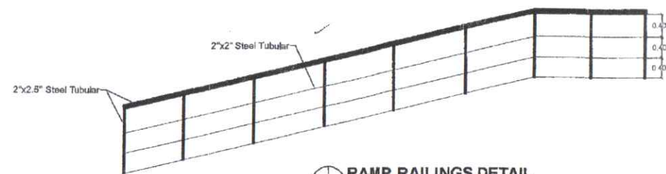
RAMP RAILINGS DETAIL Scale NTS
