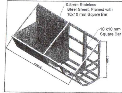
FEEDING TROUGH
