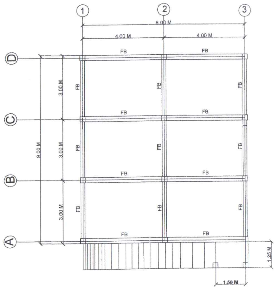
FLOOR BEAM (FB) LAYOUT Scale NTS
