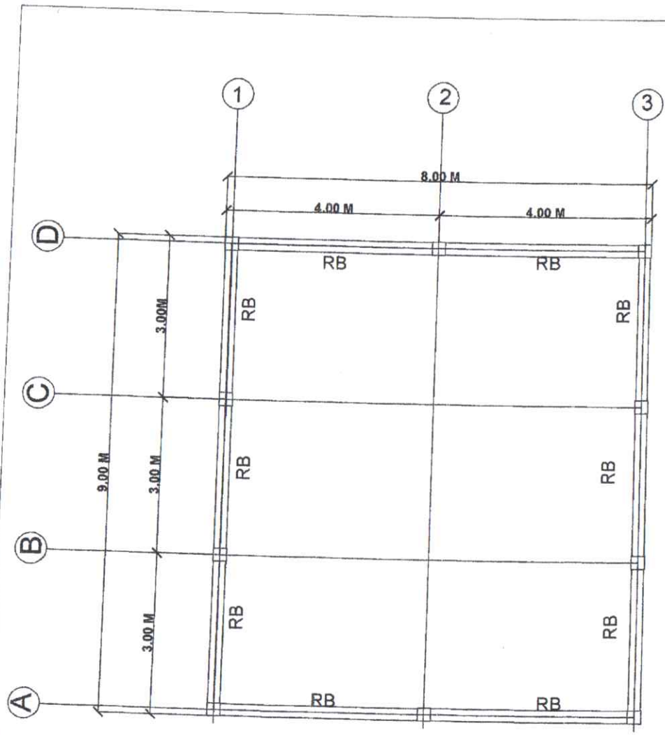
ROOF BEAM PLAN Scale NTS
