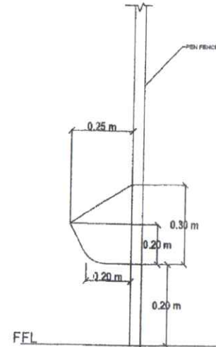
SECTION
