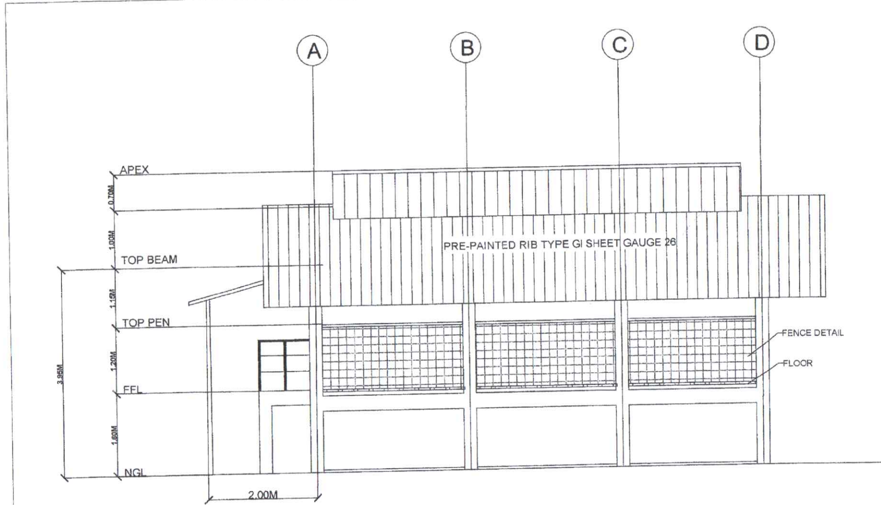
RIGHT SIDE VIEW Scale NTS
