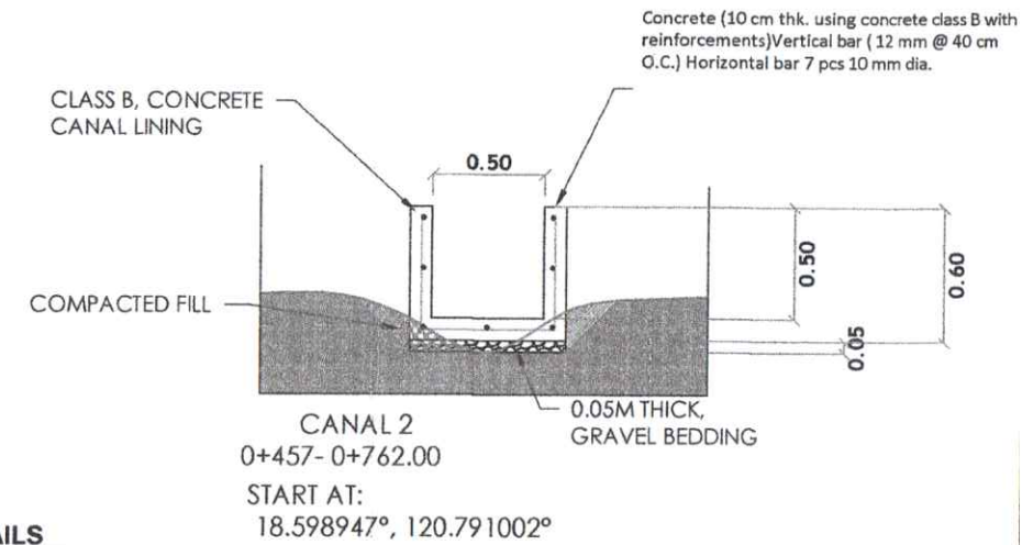
TYPICAL PLAN OF CANAL 2 SCALE 1:30
