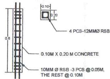
CONCRETE STIFFENER DETAILS SCALE NTS
