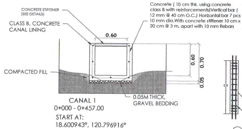
TYPICAL PLAN OF CANAL 1 SCALE 1:30
