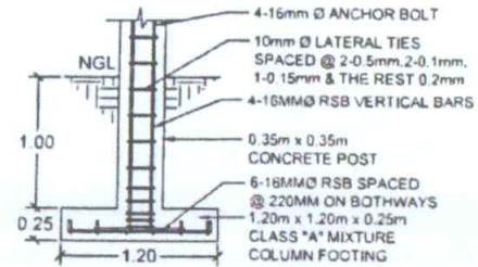
COLUMN DETAILS
