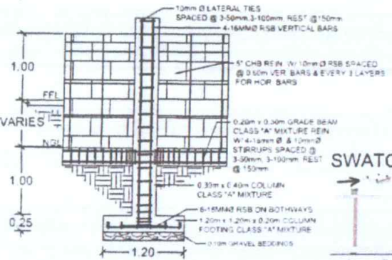
FENCE DETAILS
