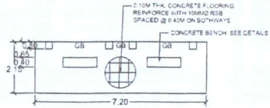
FLOOR FRAMING PLAN
