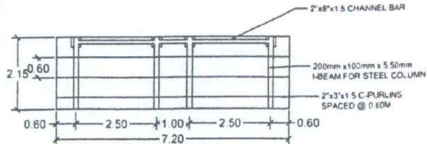
TRUSSES PLAN
