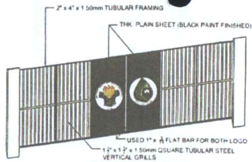
SLIDING GATE DETAILS
