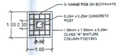
COLUMN FOOTING DETAILS, C2
