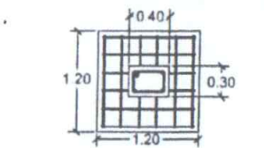
COLUMN FOOTING DETAILS
