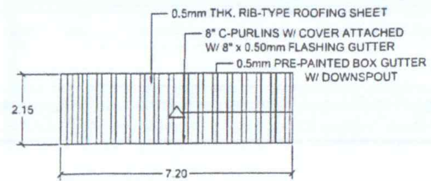
ROOF PLAN
