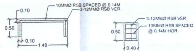
CONCRETE BENCH DETAILS
