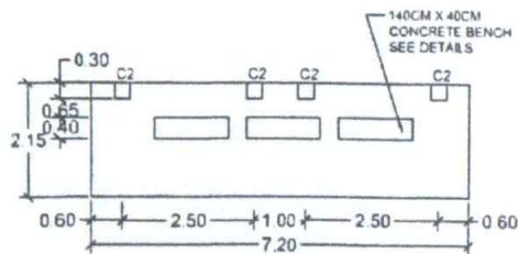
FLOOR PLAN
