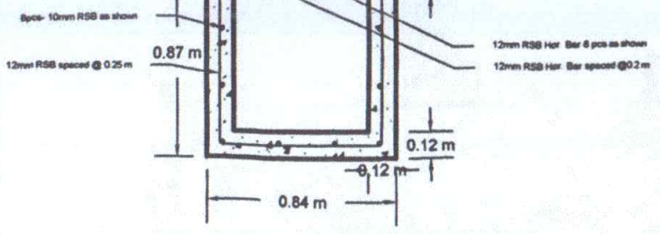
DETAILS OF CANAL WITH COVER SCALE 1:20
