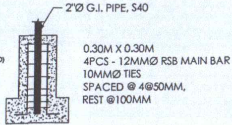
DETAIL OF CONCRETE POST SCALE 1:20
