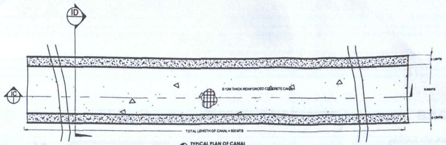
TYPICAL PLAN OF CANAL SCALE 1:20
