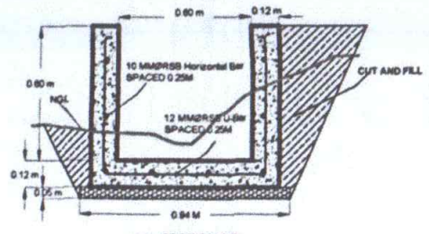
SECTION 1D SCALE 1:20
