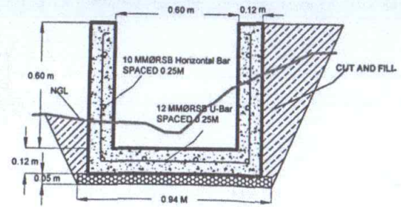
SECTION 1D SCALE 1:20
