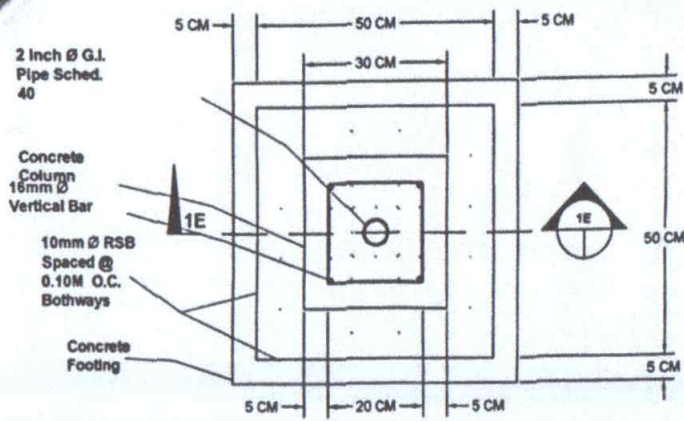
PLAN OF CONCRETE PEDESTAL SCALE: NTS
