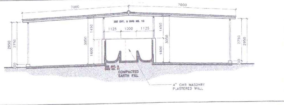
5 FEED LOT SECTION 2 SCALE: 1:100 MTS
