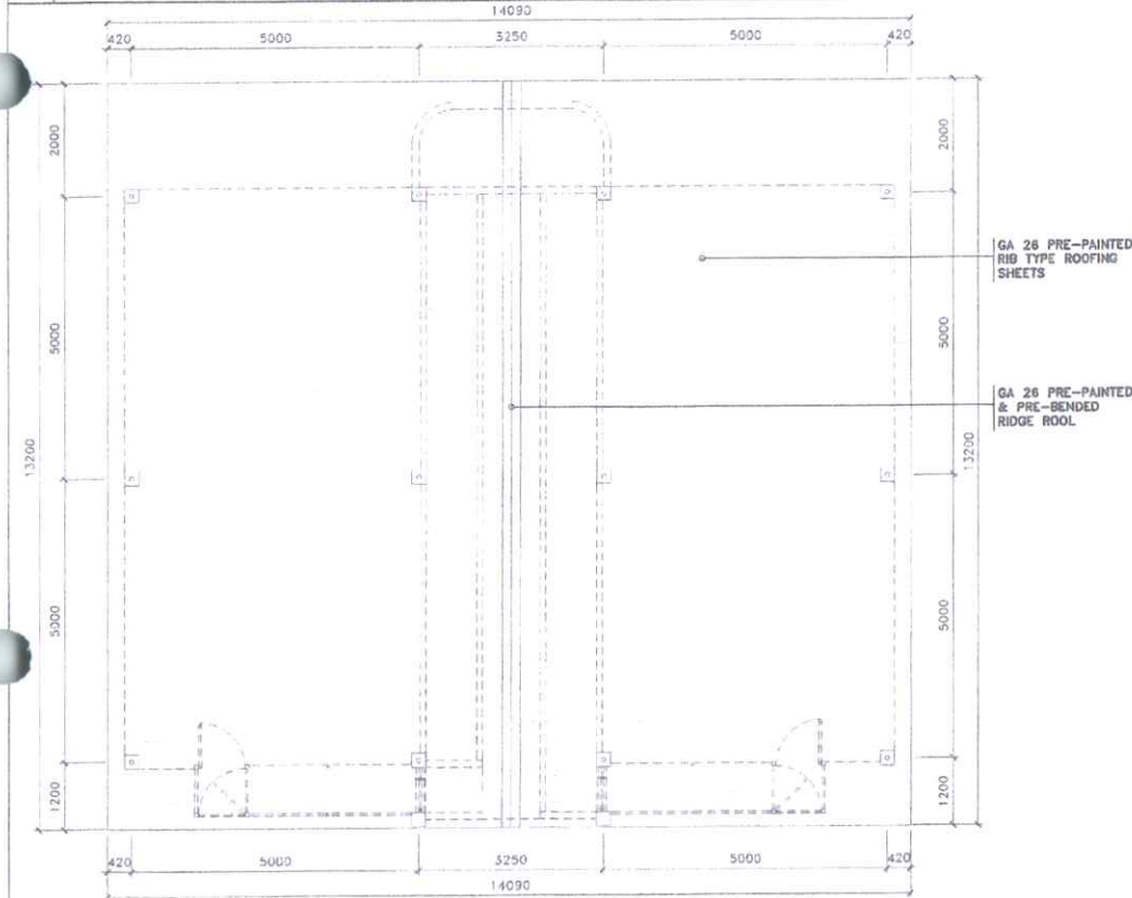
6 ROOF FINISH PLAN SCALE: 1:100 MTS
