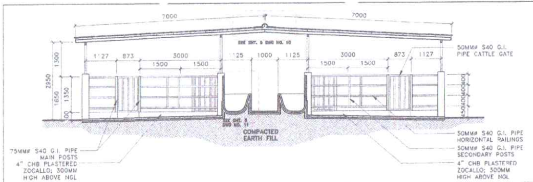
4 FEED LOT SECTION 1 SCALE: 1:100 MTS
