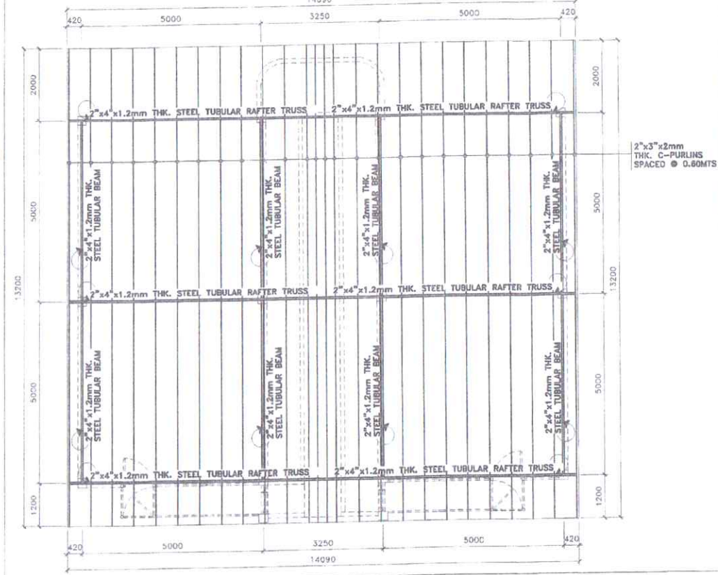
7 ROOF FRAMING PLAN SCALE: 1:100 MTS
