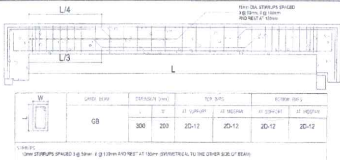
9 GRADE BEAM SCHEDULE SCALE: NTS
