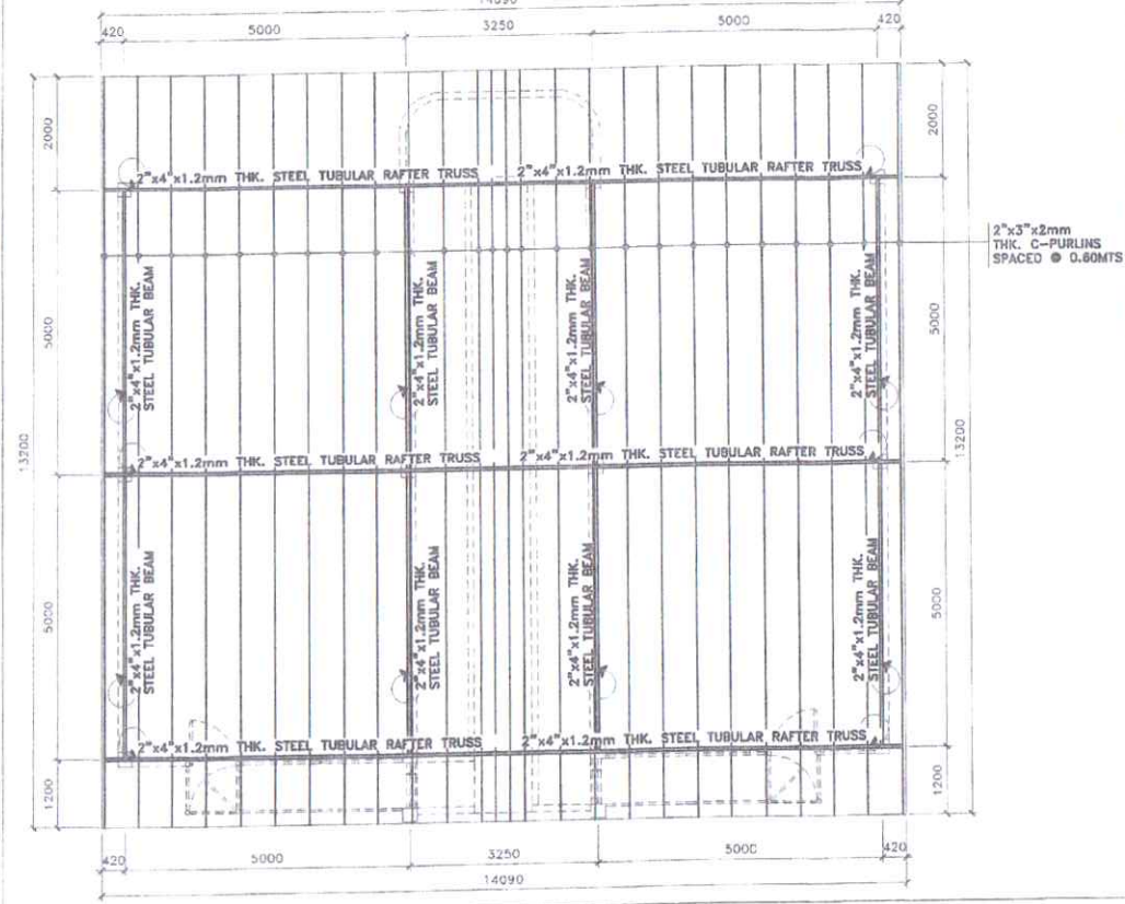
7 ROOF FRAMING PLAN SCALE: 1:100 MTS
