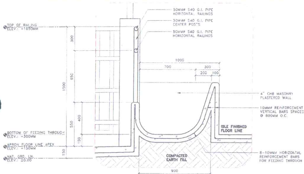
11 FEEDING THROUGH SECTIONAL DETAIL SCALE: 1:20 MTS
